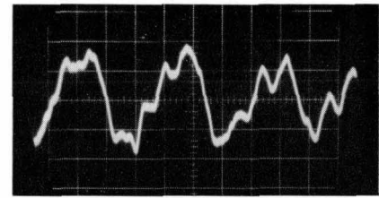
Fig. 3. Oscillogram of residual f-m in a 10 kmc measured signal made using setup of Fig. 2. Vertical sensitivity is 25 kc/division. Sweep time is 5 milliseconds/cm.
